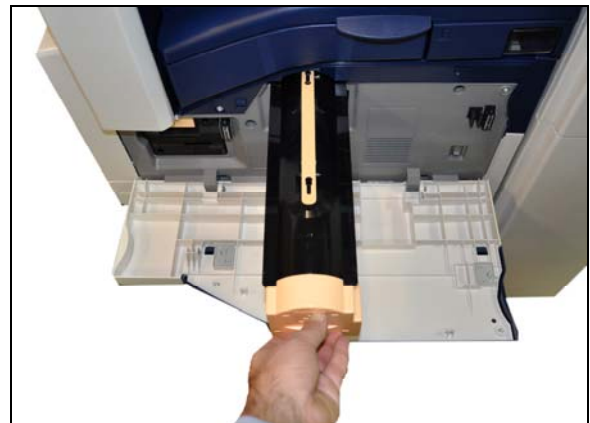
Above and below: In order to replace the Xerox WorkCentre 5335's toner cartridge the user must first open the device's front cover by pulling this panel door down. Once the door is open the user then simply slides the toner cartridge out for replacement.
