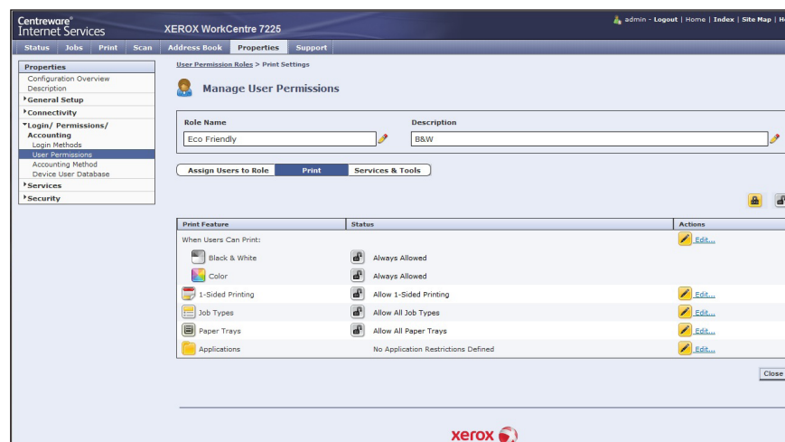
Administrators can set user permissions from the web utility.
